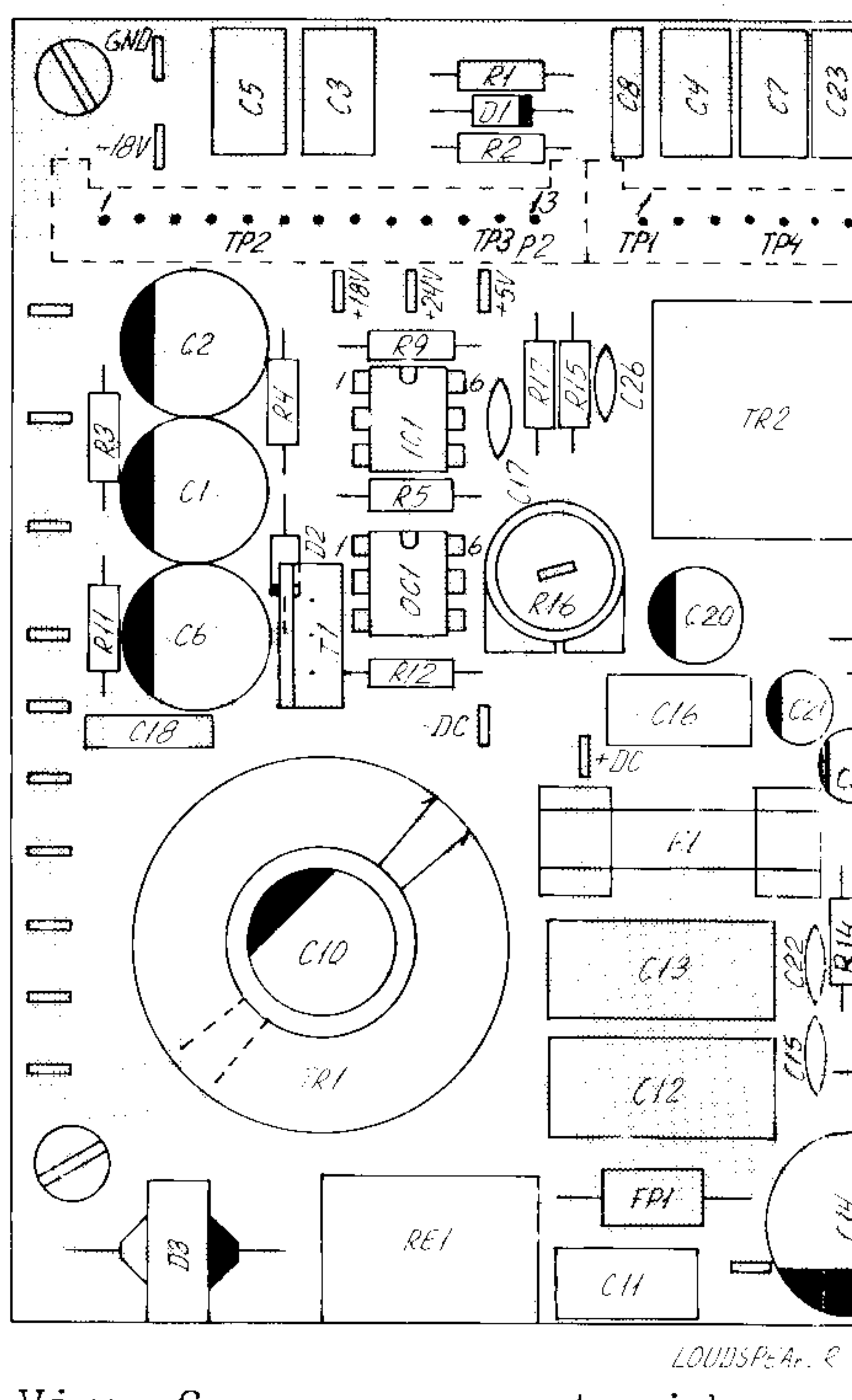
View from component side with lower side tracks.
