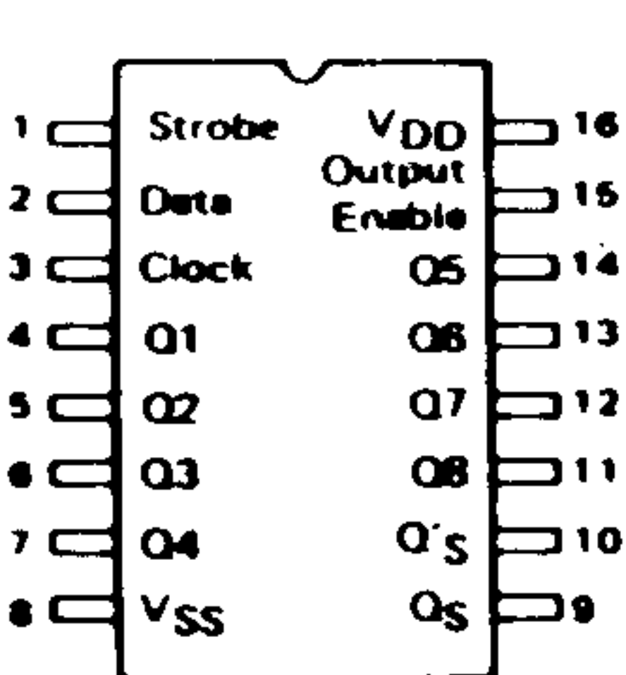
MC14094BCP
