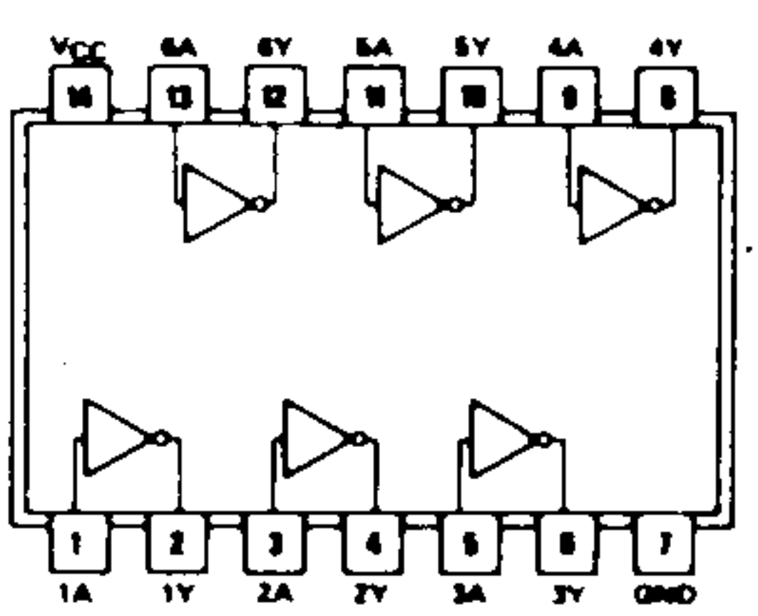
SN7406N
