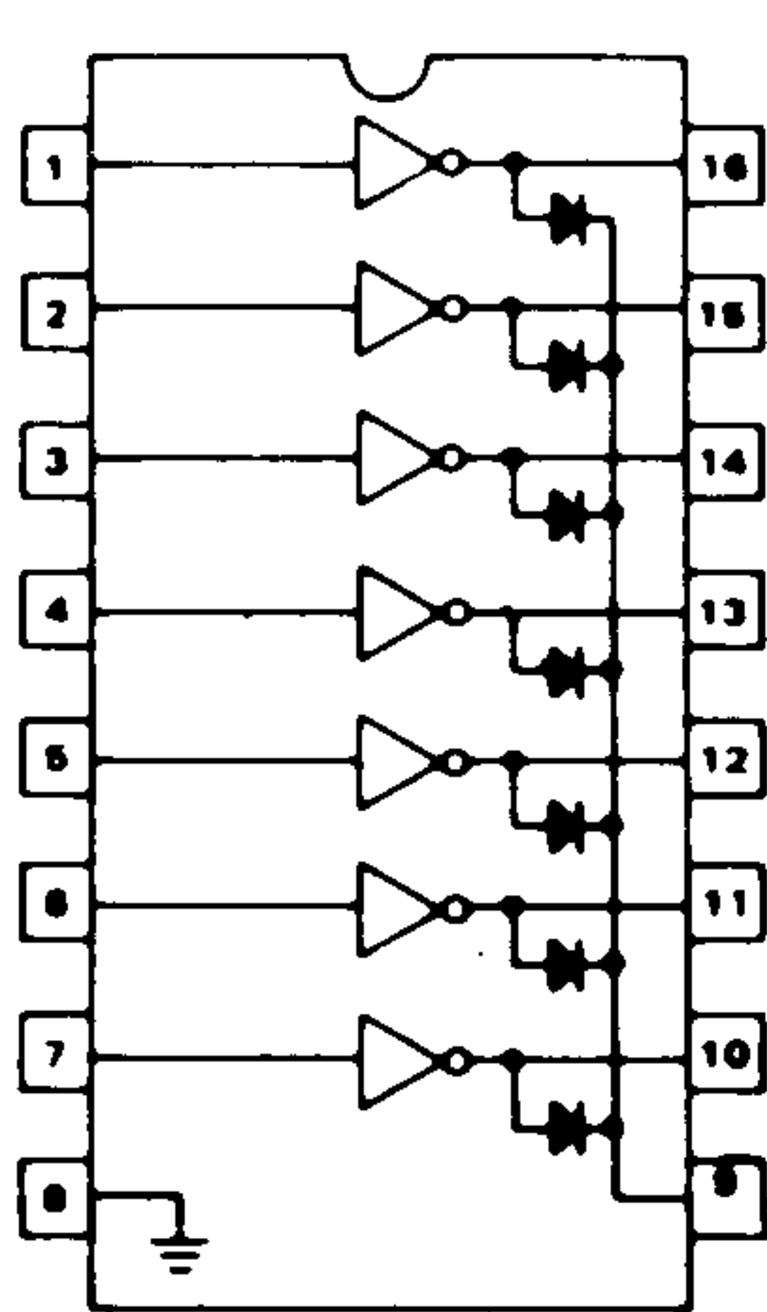
MC1413
